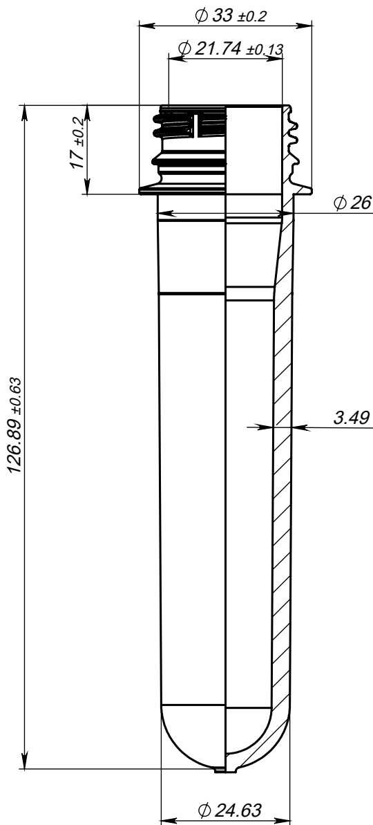
SECTION B-B
